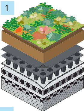
ND 4+1 Drainage System
