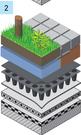
Composition Nophadrain Extensive [1] and Intensive [2] Green Roof System
