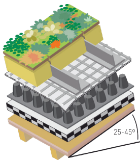
Composition Nophadrain Extensive Green Roof System – steep pitched roof
