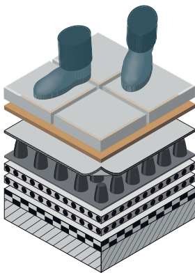
Composition Nophadrain Podium Deck System
