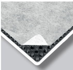
ND 220 Drainagesystem
