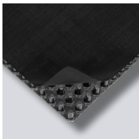
ND 600hd Drainagesystem
